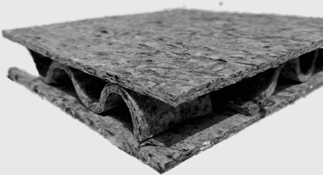
Wave-shaped core
