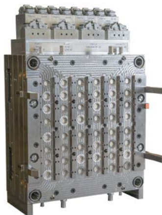
48 cavity cap mold
