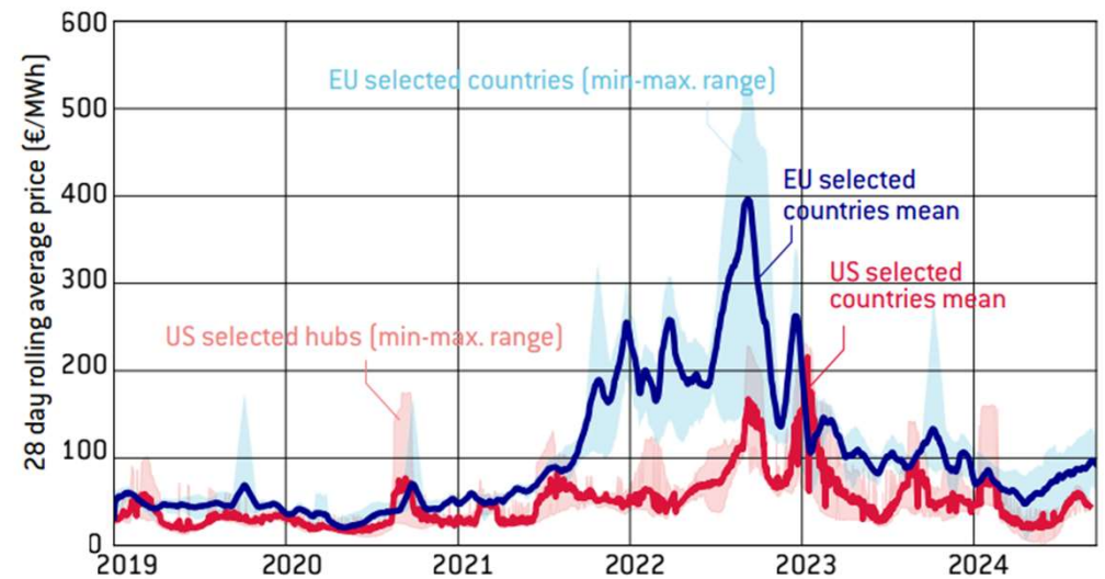
EU and US wholesale electricity prices (€/MWh)
